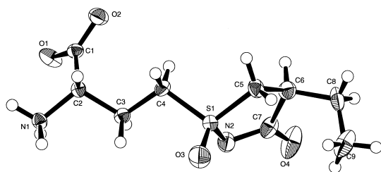
Figure 5. Structure of cyclic sulfoximine 36b as determined by X-ray diffraction analysis.
